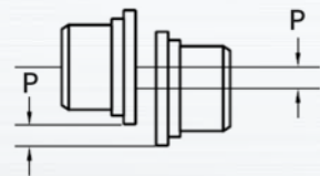
Misalignment Capacity
