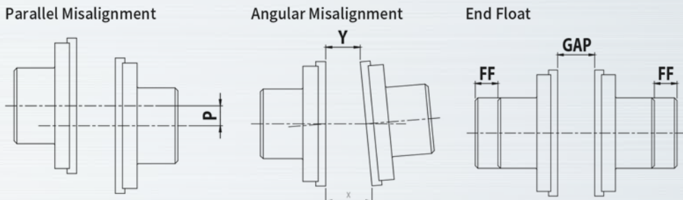
Misalignment Capacity
