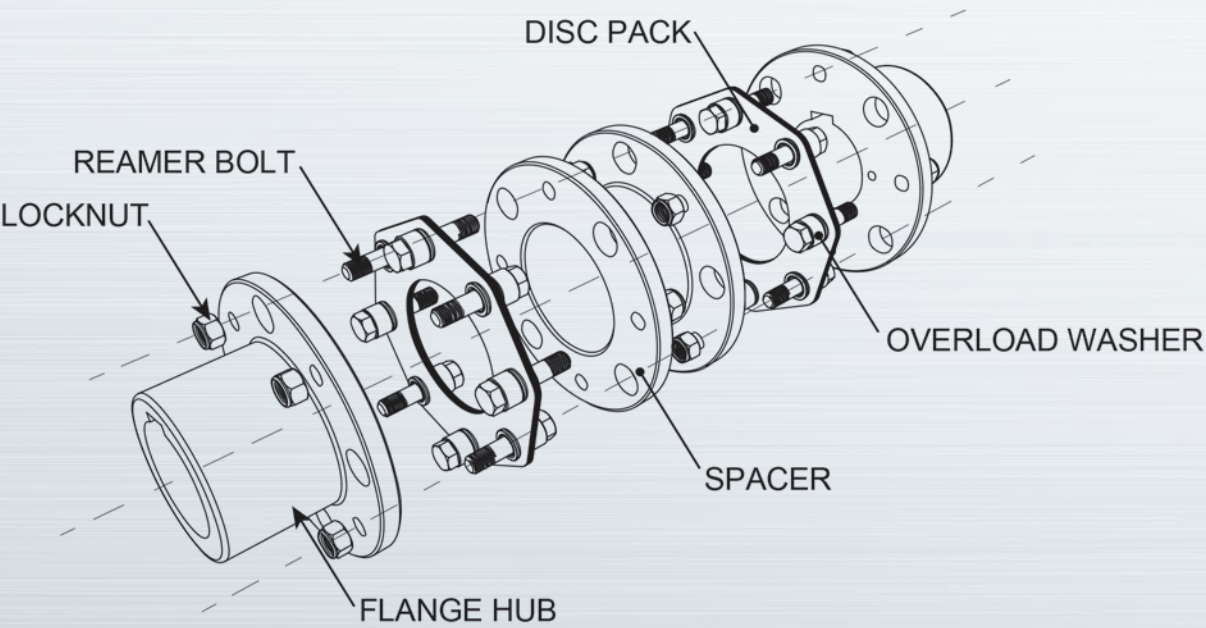
Design features of 6 - 12 bolt coupling
